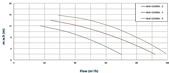
Characteristics curve
